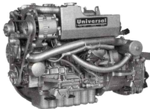
M-40B Marine Diesel Engine Shown with optional down angle transmission
